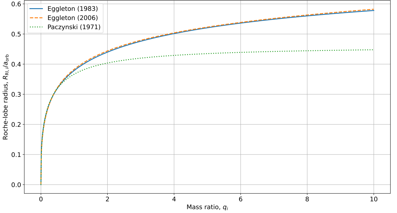
Figure 3.3: Fit of the Roche-lobe radius by Eggleton (1983) and its approximation by Eggleton (2006) (both in Eq. 3.6), compared to Paczynski (1971) , see our Eq. 3.5).
