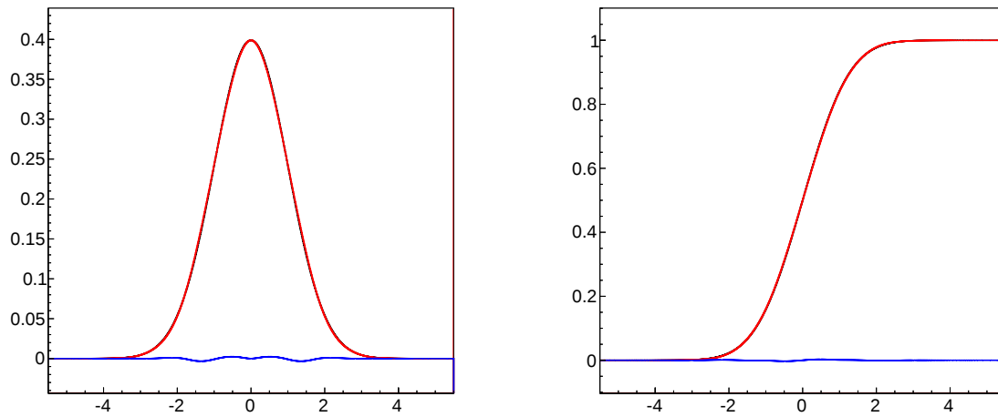
Figure 1: Left: Gauss function (analytical black; interpolated red; and differenc blue). Right: Erfc function (analytical black; interpolated red; and difference blue).
