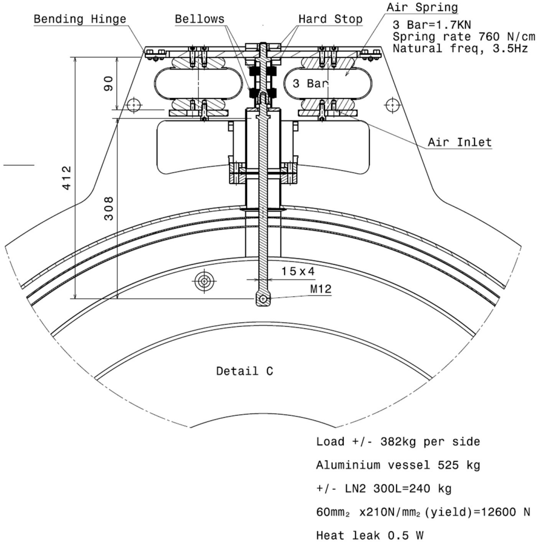
Figure 1: The cold vessel of the cryolink is suspended with air springs in order to isolate Advanced Virgo from possible bubbling noise in the LN2.
