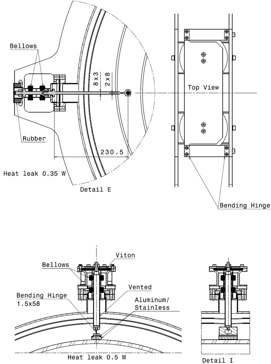
Figure 2: Suspension system for the cryolink. Left: silicon rubber spring for horizontal positioning; middle: air-spring system for vertical isolation; right: top view of the flexible hinges. See Fig. 1 for a cross section of the central air spring suspension system.
