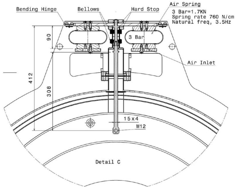
Figure 9: Schematic view of part of the suspension system for the cryolinks.
