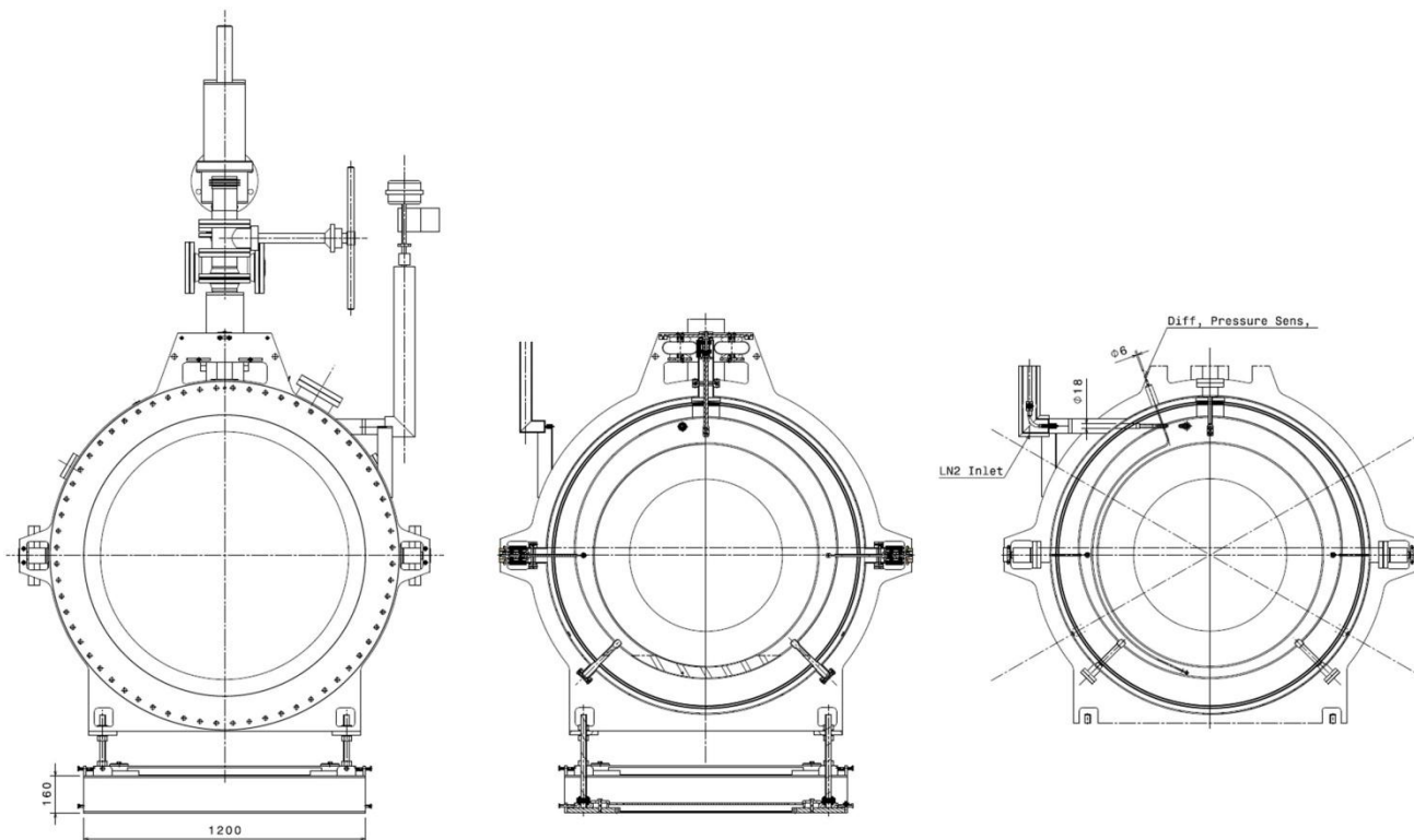
Figure 6: Cross section of the cryolink. The outer vessel of the cold link is placed off-axis with respect to the vacuum vessel. The inner vessel of the cold link is placed on-axis.
