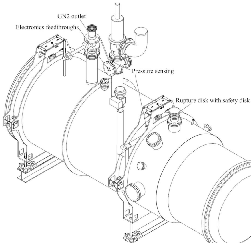
Figure 2: Cryolink with internal baffles for shielding the mirror from direct view of the cold surface. Internal baffles are shown as example of feasibility. The optimal solution for the discussed light mitigation is to be studied.
