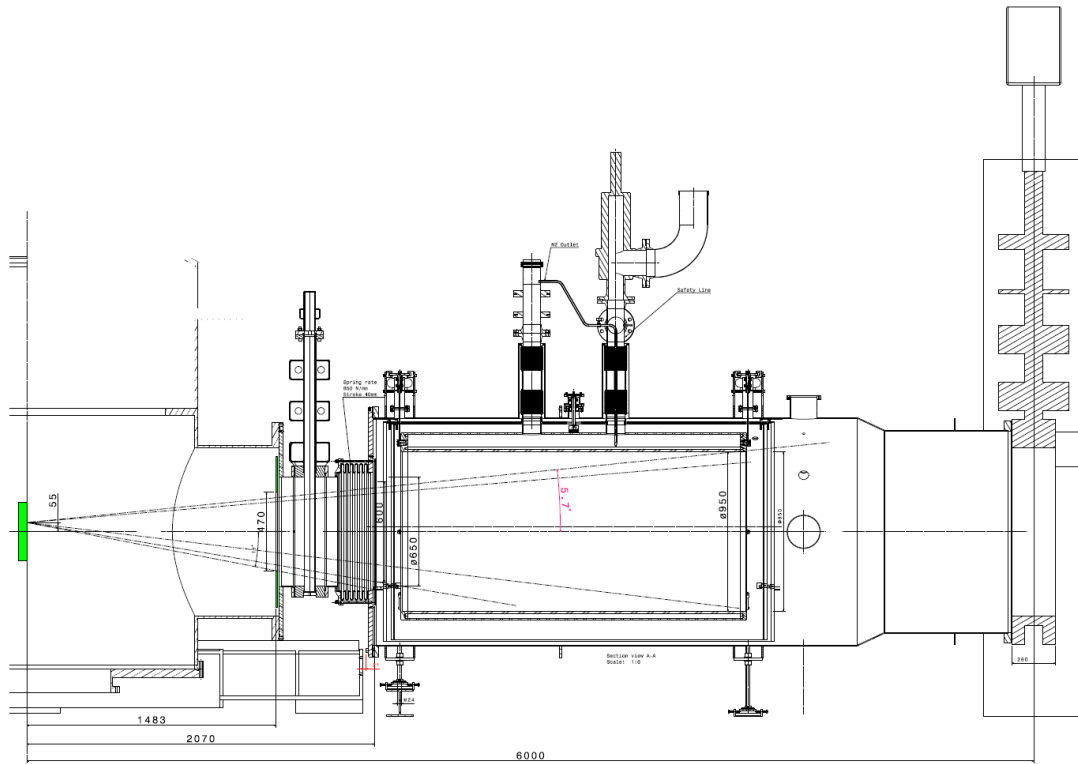
Figure 2: Cryolink with internal baffles for shielding the mirror from direct view of the cold surface. Internal baffles are shown as example of feasibility. The optimal solution for the discussed light mitigation is to be studied.
