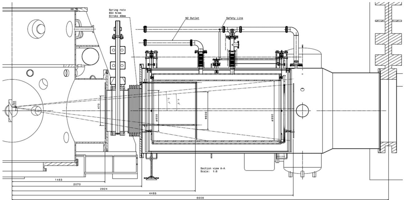
Figure 2: Cryolink with internal baffles for shielding the mirror from direct view of the cold surface. Internal baffles are shown as example of feasibility. The optimal solution for the discussed light mitigation is to be studied.
