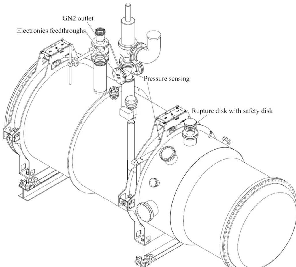
Figure 3: Isometric view of a cryolink for Advanced Virgo. The reinforcement rings and the suspension system is visible. At the top the large nitrogen exhaust lines can be seen.
