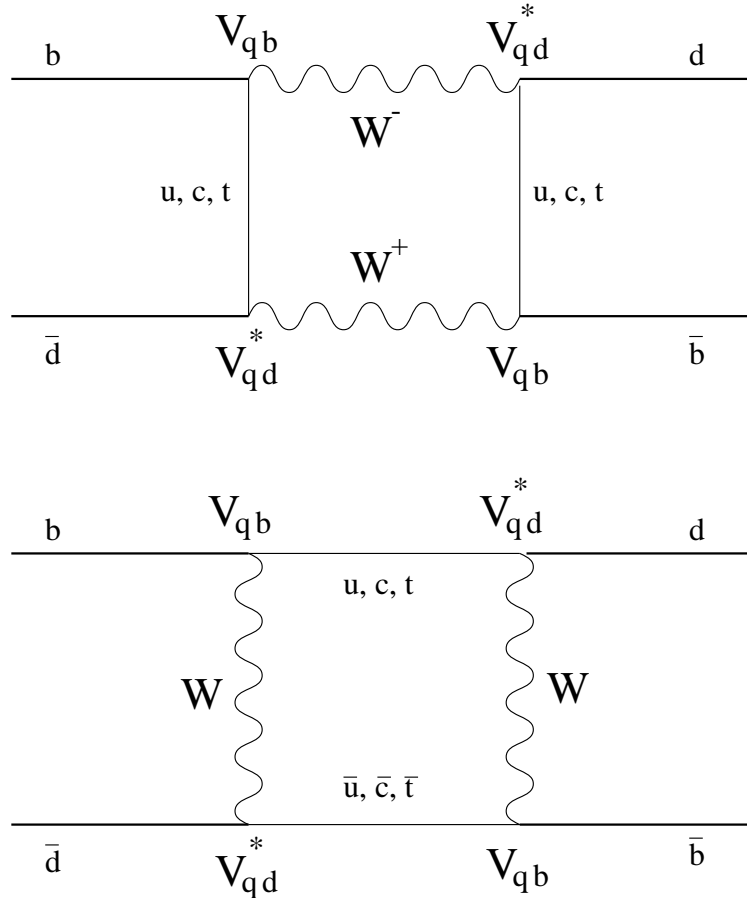
Figure 45: Mixing diagrams for B -mesons. The corresponding CKM entries are shown.
