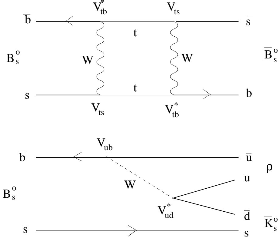
Figure 50: B_s -mixing and tree diagrams contributing in the decay B_s^0 \rightarrow \rho K_S .
