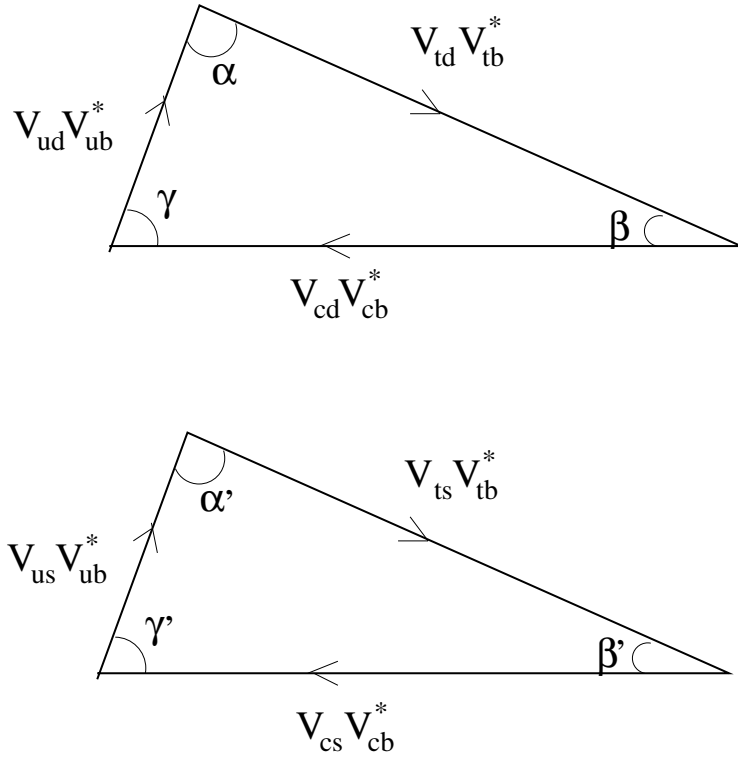
Figure 29: Representation in the complex plane of the triangle formed by the CKM matrix elements of the first and third columns.
