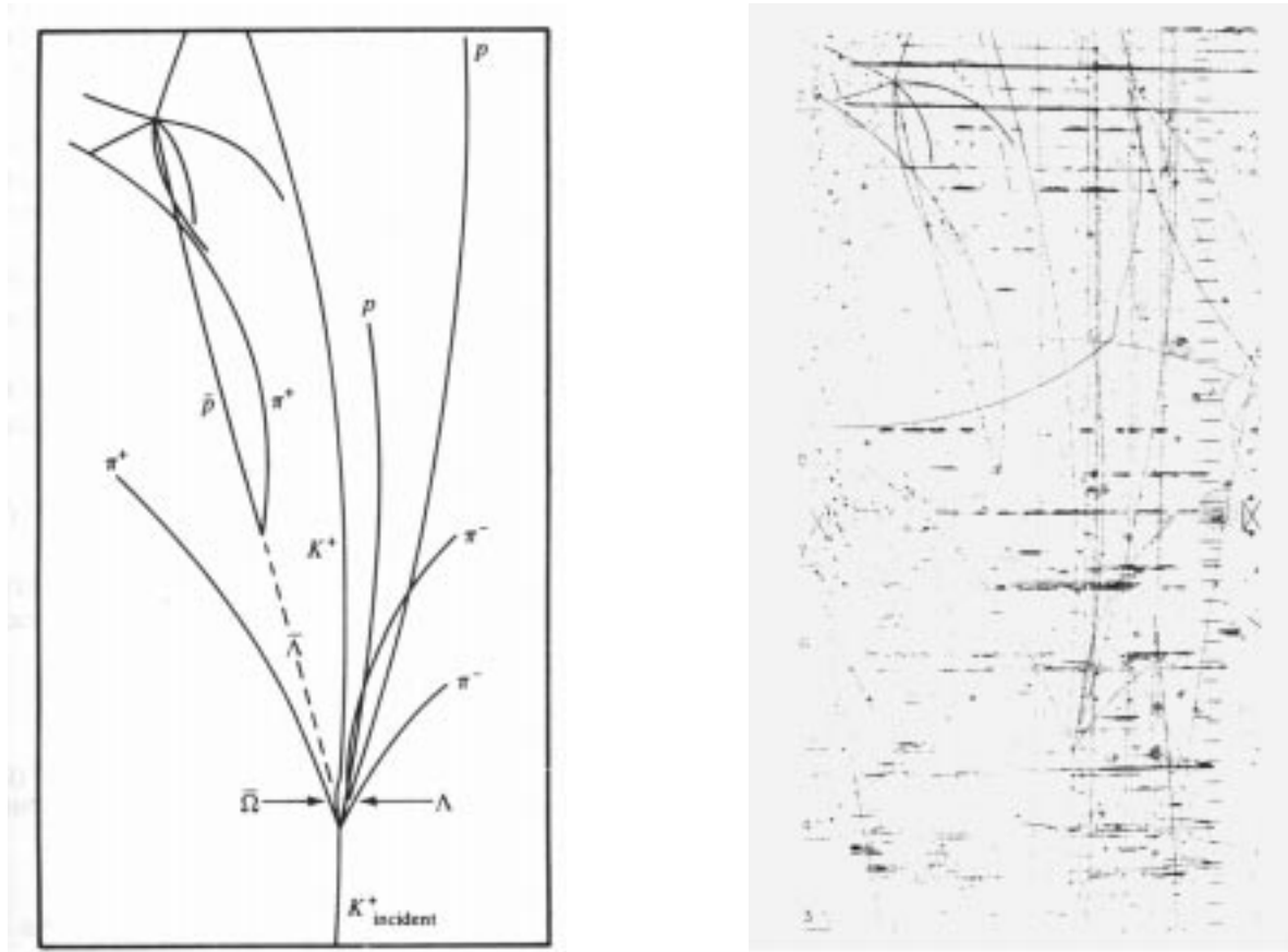
Figure 10: Sketch (left) and bubble chamber picture (right) for the reaction K^+d \rightarrow \bar{\Omega}\Lambda p\pi^+\pi^- observed in the study of K^+d -interactions at a momentum of 12 GeV/c using the two-mile linear accelerator of the Stanford Linear Accelerator Center.
