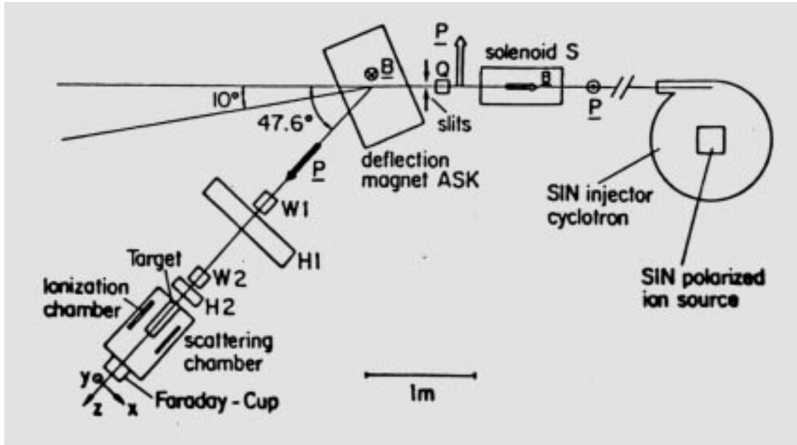
Figure 8: Experimental set up for the measurement of parity violation in proton-proton scattering. Longitudinal polarized protons with an energy of 50 MeV are scattered from hydrogen.
