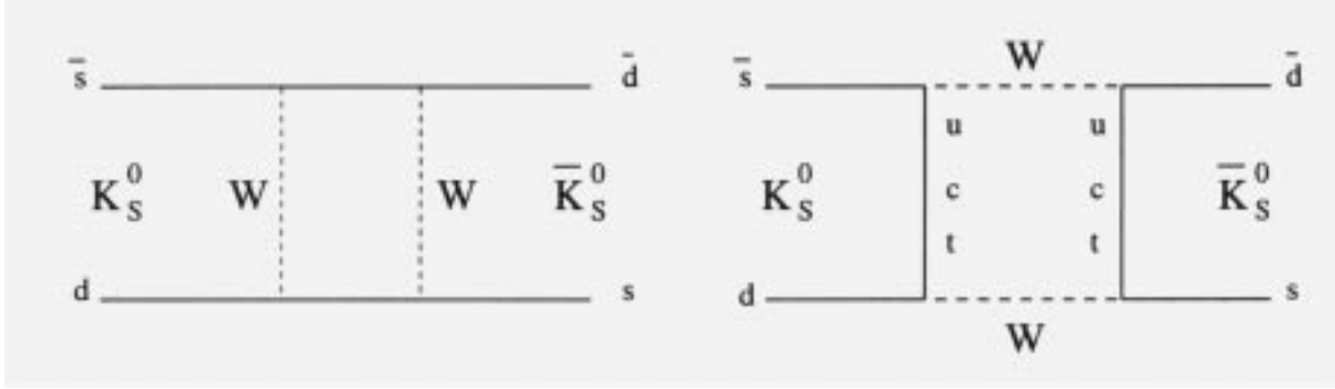
Figure 36: Mixing of K^0 \leftrightarrow \bar{K}^0 due to the weak interaction. Note that the strangeness changes by two units.
