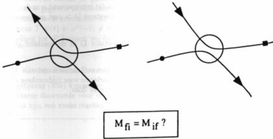
Figure 11: Schematic representation of time reversal invariance in a two-particle collision.
