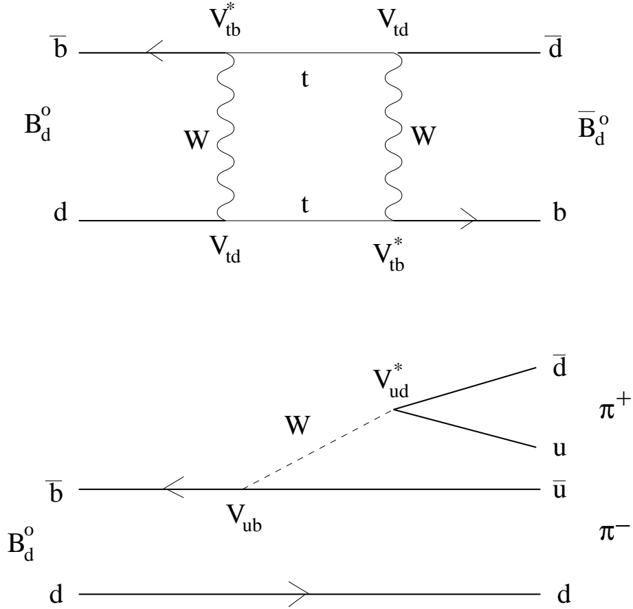
Figure 49: B_d -mixing and tree diagrams contributing in the decay B_d^0 \rightarrow \pi\pi .
