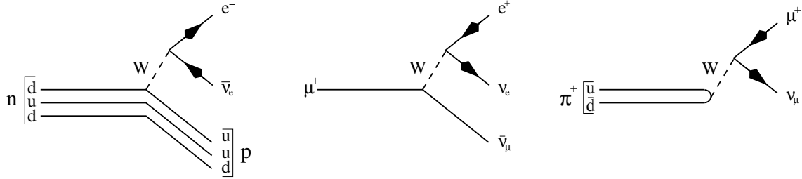
Figure 23: (a) Charged-current decay n \rightarrow pe^- \bar{\nu}_e , \mu^+ \rightarrow e^+ \bar{\nu}_\mu \nu_e , and \pi^+ \rightarrow \mu^+ \nu_\mu .
