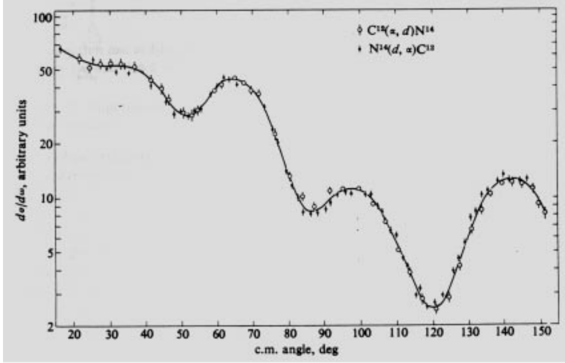
Figure 12: Comparison of the cross section for the reaction ^{14}\text{N}(d, \alpha)^{12}\text{C} and its inverse reaction ^{12}\text{C}(\alpha, d)^{14}\text{N} .
