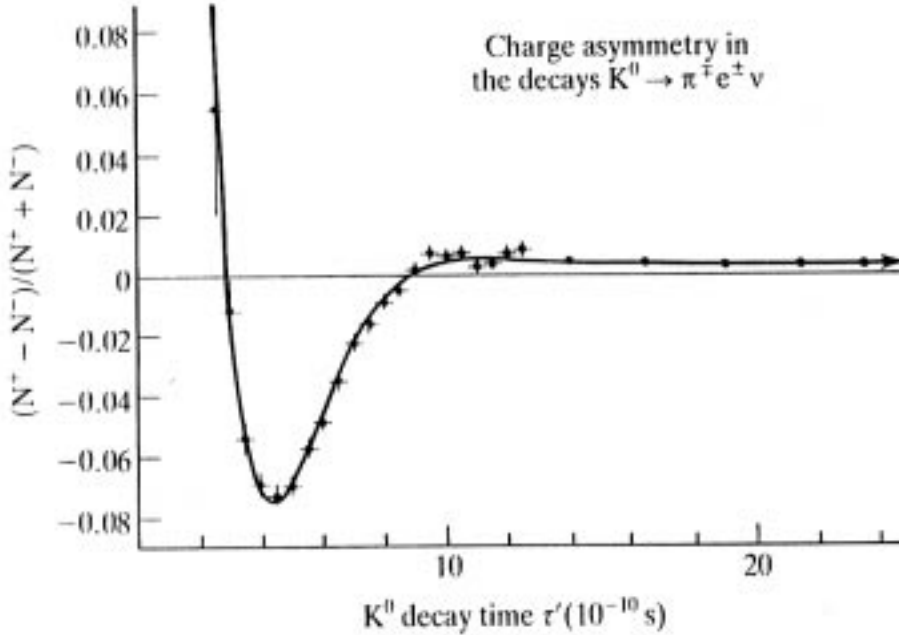
Figure 42: Charge asymmetry for semileptonic decay of neutral kaons (from Ref. [4]).
