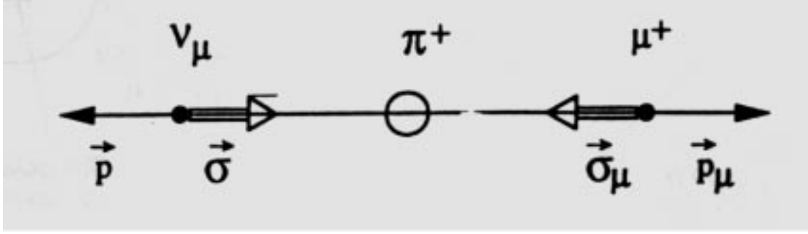
Figure 7: Schematic representation of the helicities in the decay of a positively charged pion into a muon and muon neutrino.
