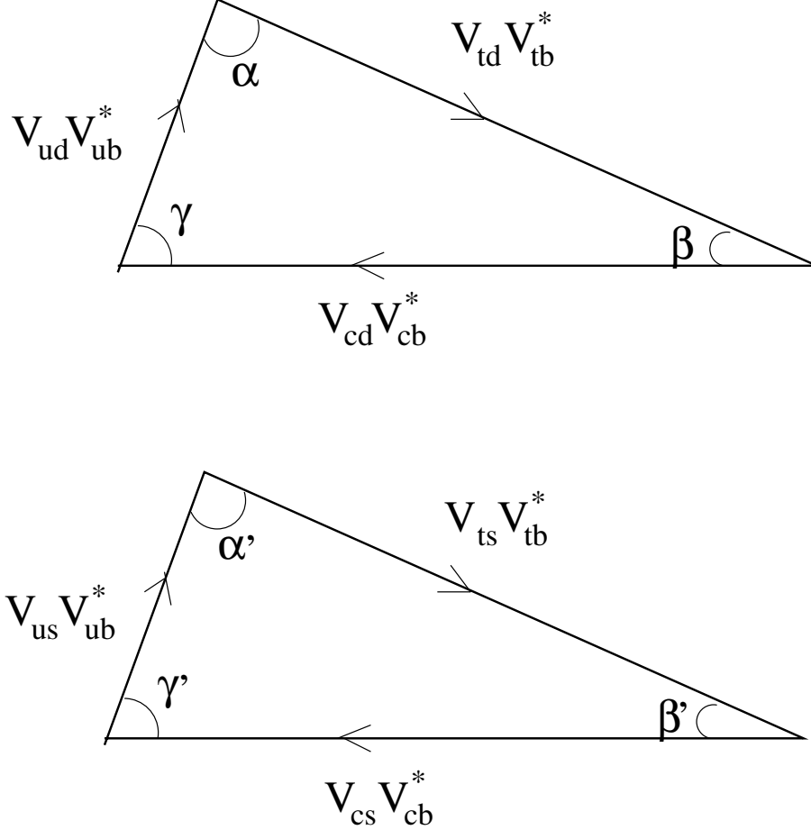
Figure 46: Two unitarity triangles which provide the measurable angles in B -physics.
