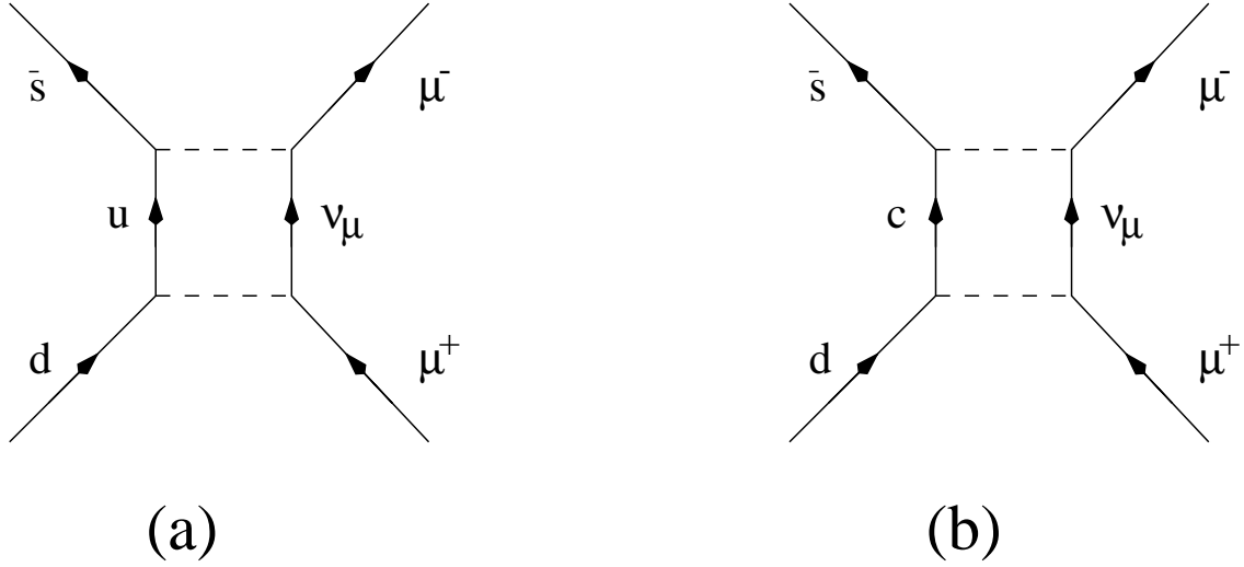
Figure 26: Second-order contributions to the neutral-current decay K_L^0 \rightarrow \mu^+\mu^- . (a) Feynman diagram with an intermediate u quark; (b) intermediate c quark.
