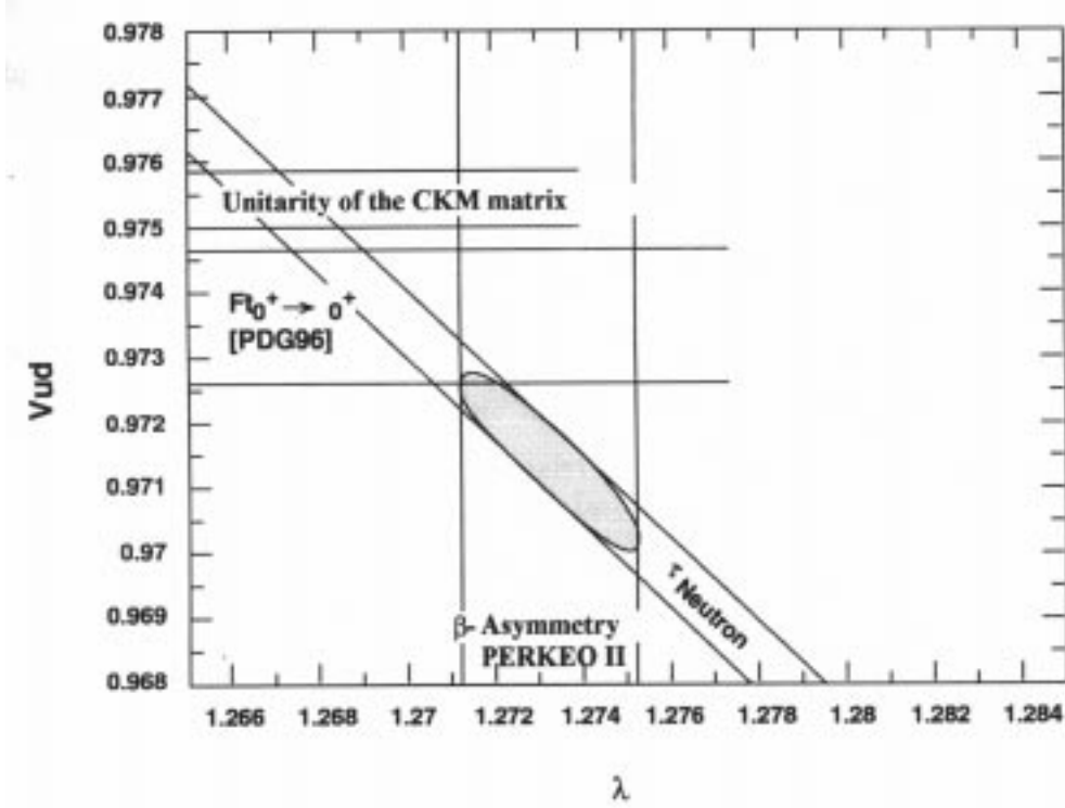
Figure 28: Determination of the CKM matrix element V_{ud} from measurement of the neutron life time.
