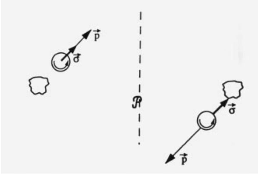
Figure 5: Helicity of particles that are emitted by an unpolarized source. The figure on the right-hand side shows the situation after a parity transformation.
