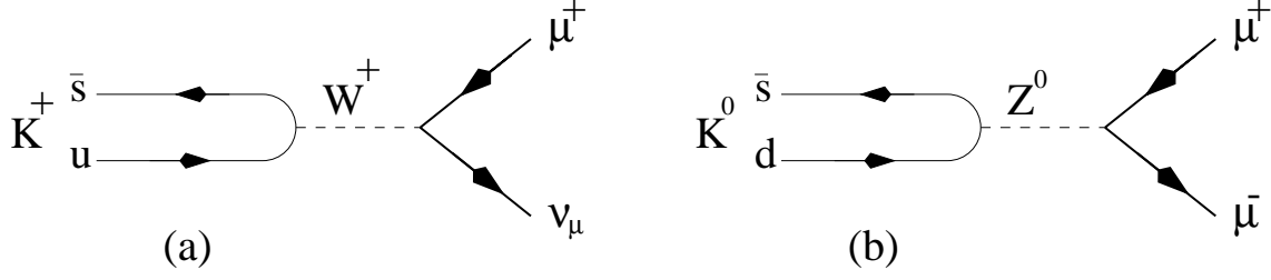
Figure 25: (a) Charged-current decay K^+ \rightarrow \mu^+ \nu_\mu ; (b) neutral-current decay K_L^0 \rightarrow \mu^+ \mu^- .
