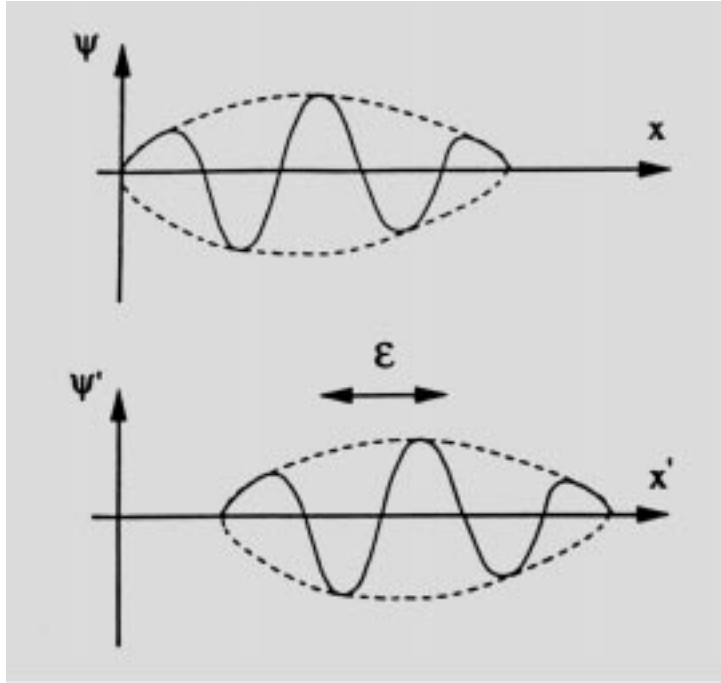
Figure 1: Illustration of a continuous symmetry transformation through the translation of the wave function of a particle.
