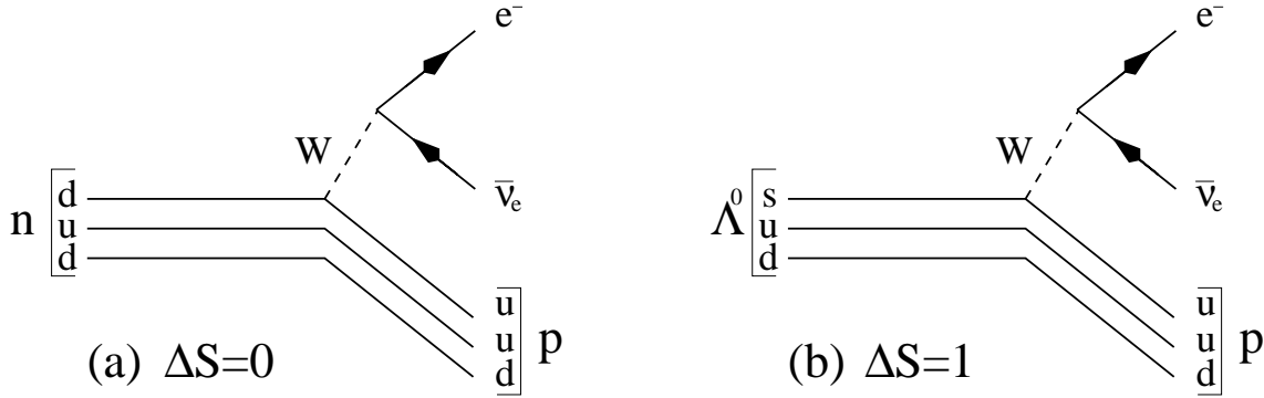
Figure 24: (a) Strangeness conserving charged-current decay n \rightarrow pe^- \bar{\nu}_e ; (b) Strangeness changing charged-current decay \Lambda^0 \rightarrow pe^- \bar{\nu}_e .
