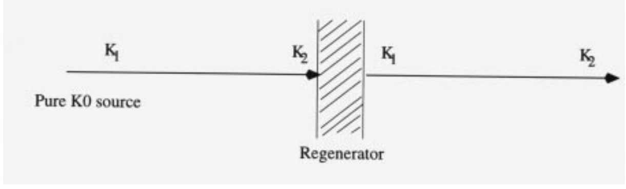
Figure 35: Schematic representation of the phenomenon of regeneration of K_S -mesons from a beam of K_L -mesons.
