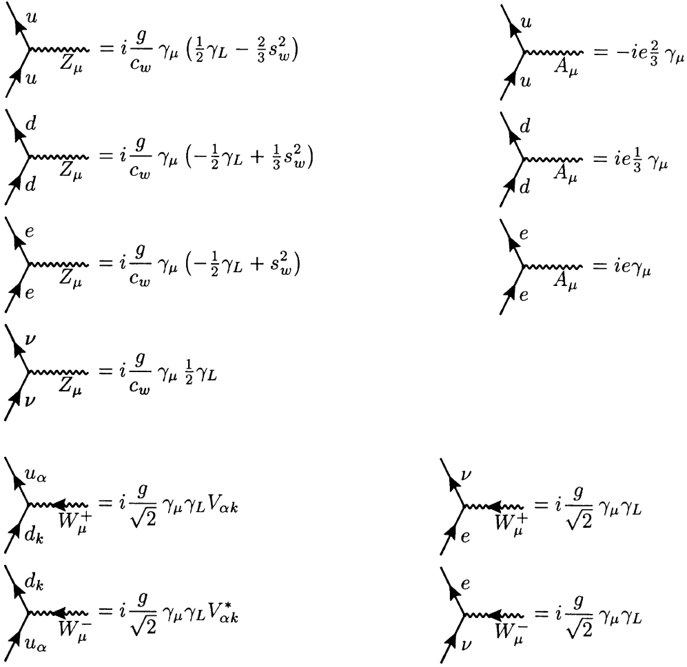
Figure 21: Gauge interactions of the fermions in the standard model.
