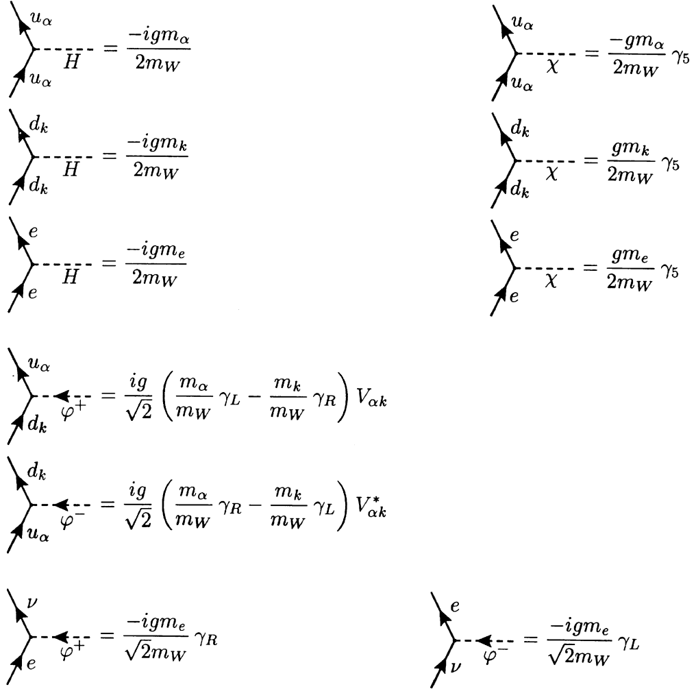
Figure 22: Yukawa couplings of the fermions.
