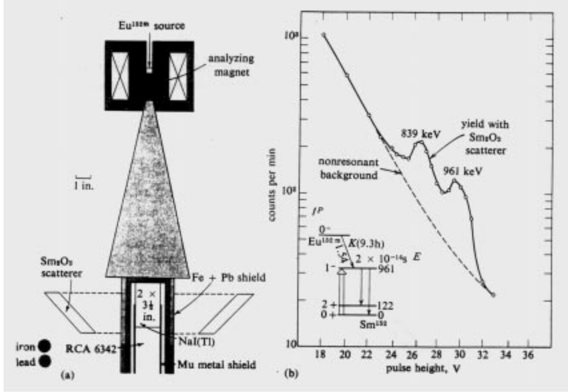
Figure 6: Experimental set up used by Goldhaber, Grodzins and Sunyar to demonstrate that the helicity of neutrinos, emitted in the decay of ^{152}\text{Eu} , is negative. The analyzer magnet selects the circular polarization of the photons, The \text{Sm}_2\text{O}_3 scatters through nuclear fluorescence radiation to the NaI detector.
