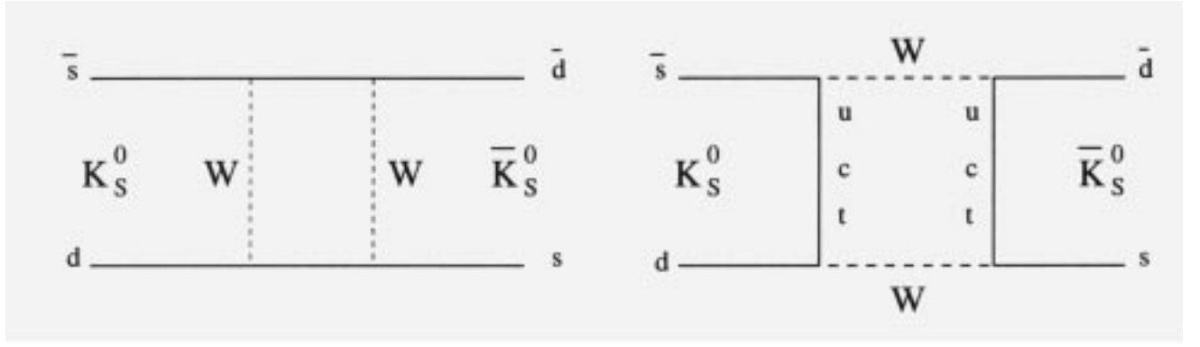
Figure 43: Mixing\ of\ K^0 \leftrightarrow \bar{K}^0\ due\ to\ the\ weak\ interaction. Note that the strangeness changes by two units.
