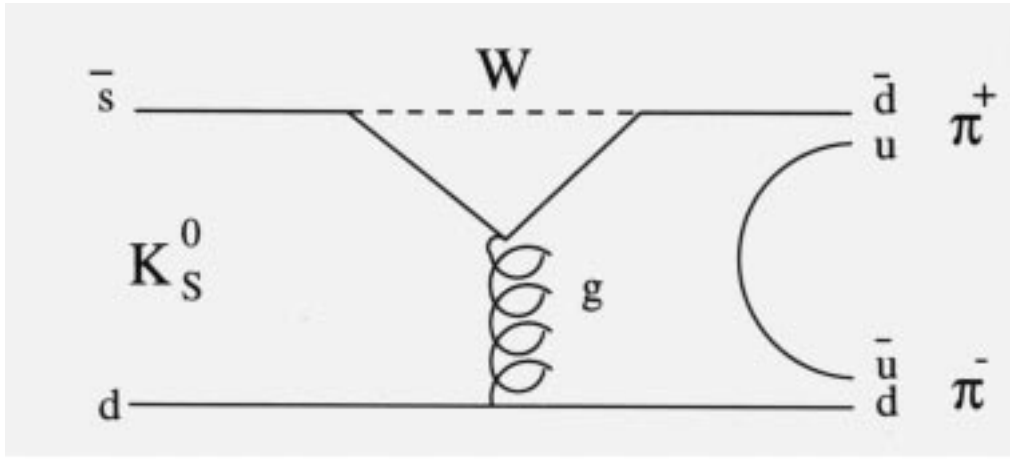
Figure 40: Penguin amplitude that plays a role in direct CP violation in the decay of kaons. Note that the strangeness changes by one unit.
