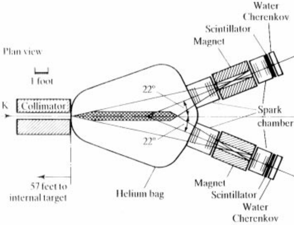
Figure 37: Schematic representation of the experimental set-up used by Christenson, Cronin, Fitch and Turlay to demonstrate \mathcal{CP} -violation in K_L -decay.
