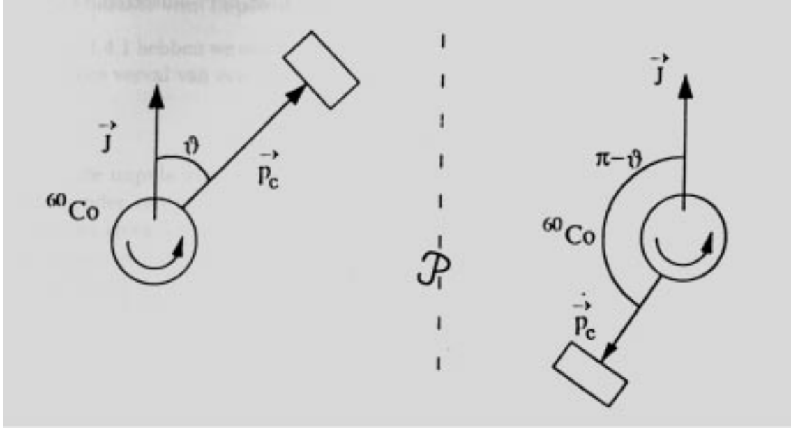
Figure 3: Schematic representation of the experimental set up used by Wu and collaborators to demonstrate the violation of parity in the \beta -decay of ^{60}\text{Co} .
