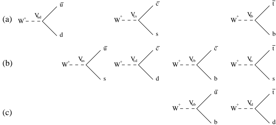
Figure 27: The CKM matrix elements are related to the strength of the coupling of the electroweak charged currents to different quark flavors. The diagrams can be organized as follows: a) Cabibbo allowed, b) Cabibbo suppressed, and c) almost forbidden transitions.
