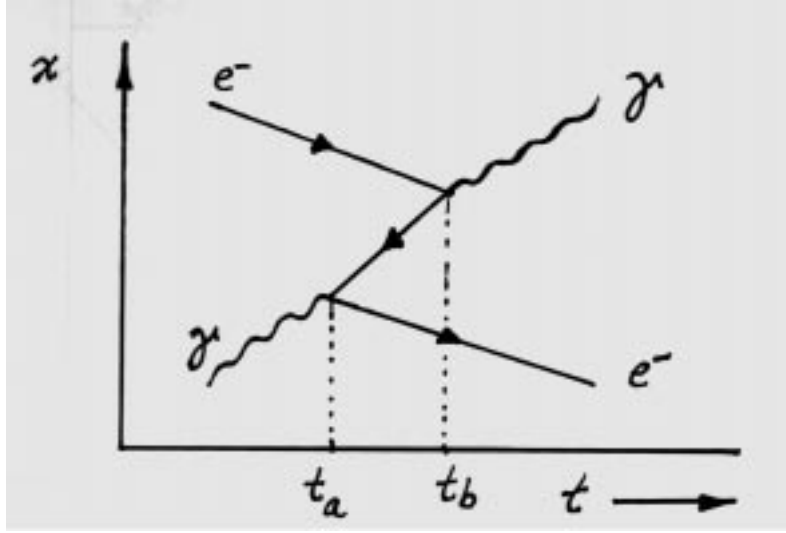
Figure 9: Motion of a particle and antiparticle in the Feynman diagram for photon-electron scattering.
