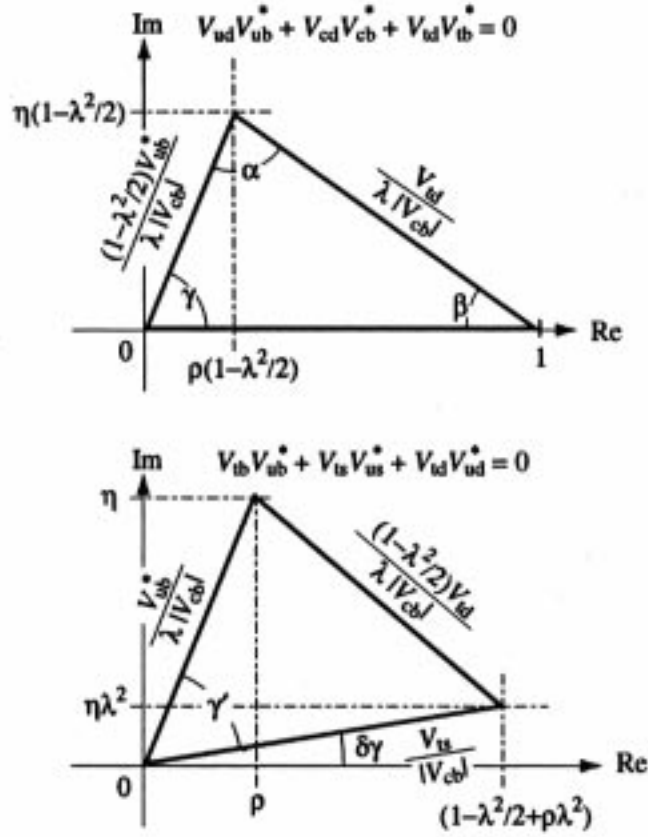
Figure 30: Representation in the complex plane of the triangle formed by the CKM matrix elements of the first and third columns. The triangle has been rescaled.
