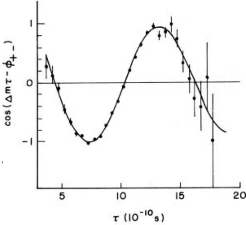
Figure 33: Strangeness oscillations and the interference term. From the fit one can determine the K_2^0 - K_1^0 mass difference \Delta m and the phase \phi_{+-} between both amplitudes.
