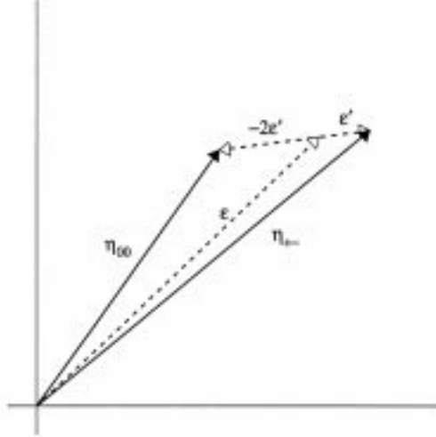
Figure 39: Schematic representation of the various complex amplitudes that play a role in the description of \mathcal{CP} violation in the decay of kaons.
