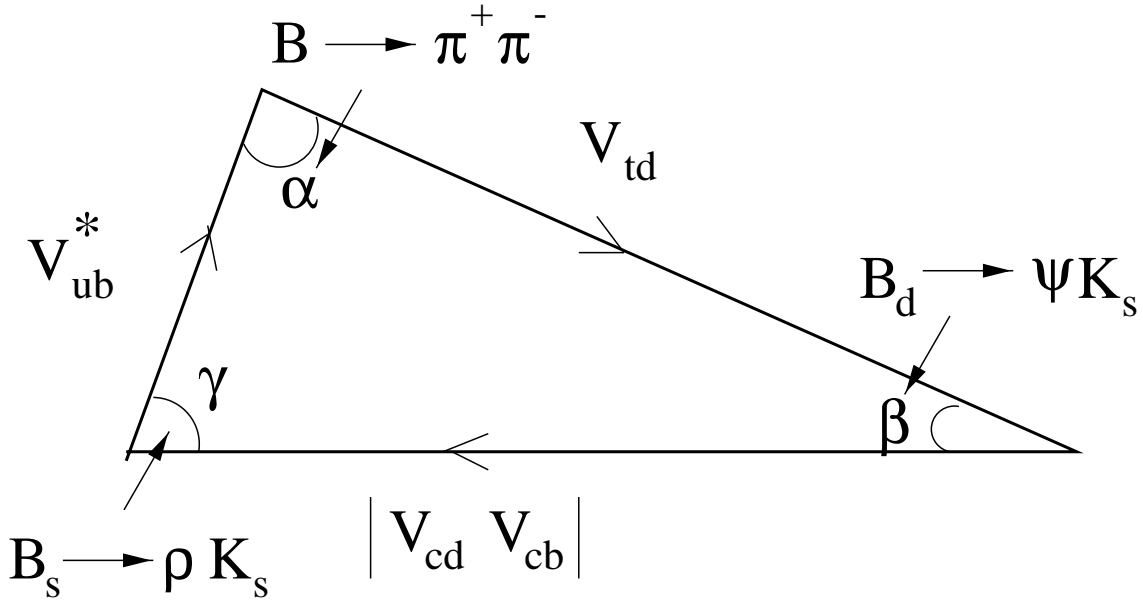
Figure 44: The unitarity triangle is a representation in the complex plane of the triangle formed by the CKM matrix elements V_{ud}V_{ub}^* , V_{cd}V_{cb}^* and V_{td}V_{tb}^* .
