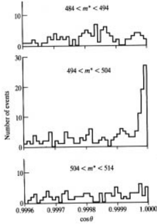
Figure 38: Angular distribution of pions with opposite charge from the decay K_2^0 \rightarrow \pi^+ \pi^- versus \cos \theta for three mass ranges.
