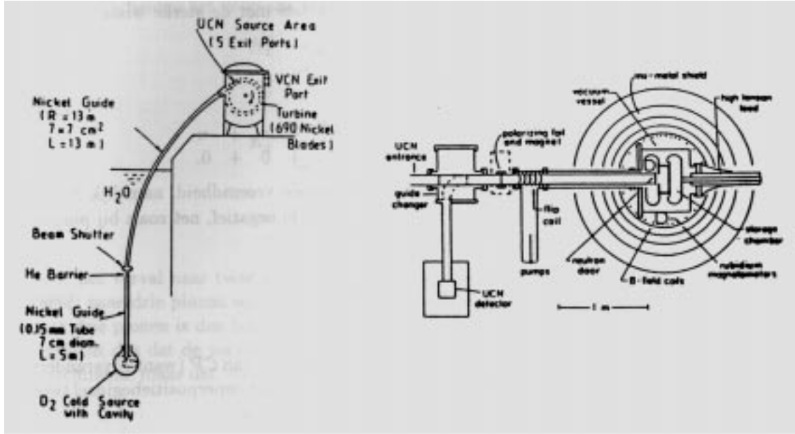
Figure 13: Experimental set up used for the determination of the electric dipole moment of the neutron.
