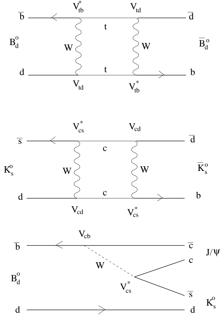
Figure 48: B_d -mixing, K -mixing and tree diagrams contributing in the decay B_d^0 \rightarrow J/\psi K_S .
