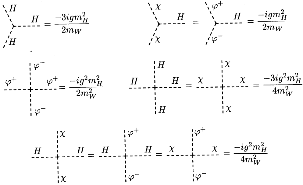
Figure 14: Self-interactions of the Electroweak gauge bosons.
