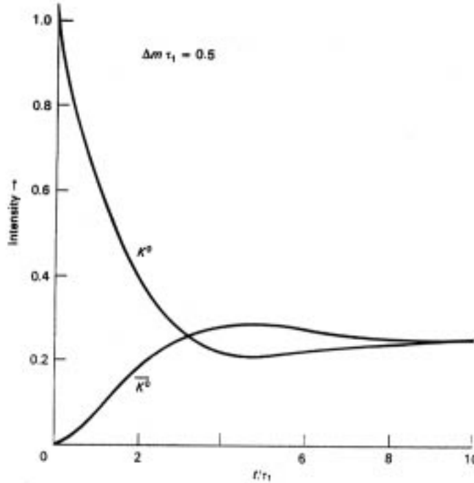
Figure 31: A beam initially consisting of only K^0 -mesons transforms after a certain time into a K_2^0 beam, that contains equal amounts of K^0 and \bar{K}^0 .
