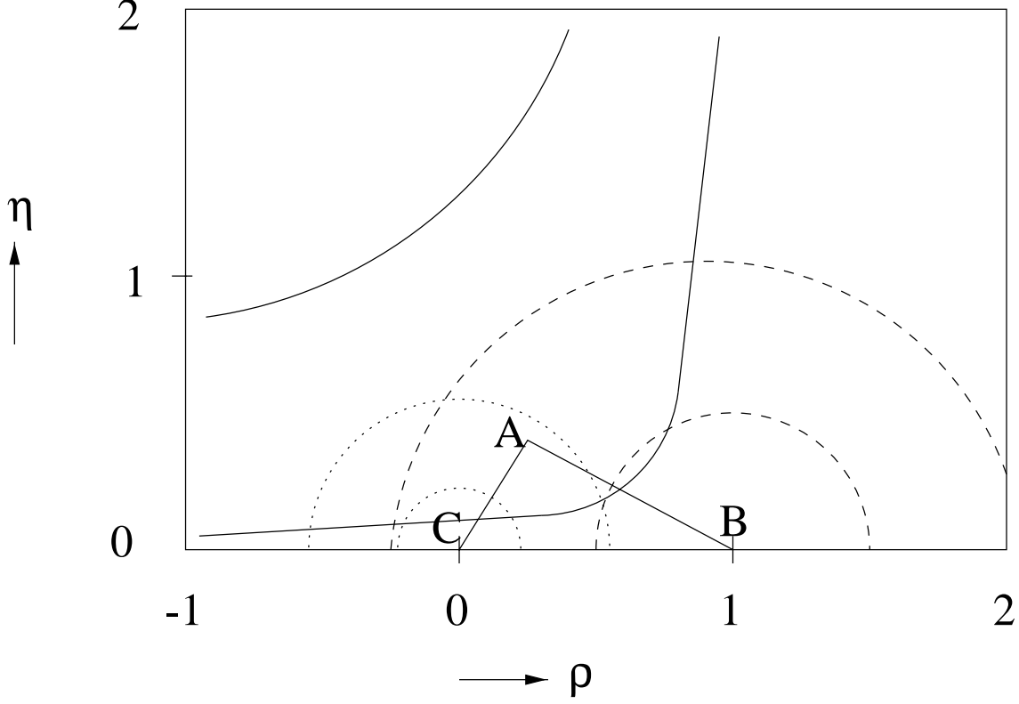
Figure 47: Constraints in the (\rho, \eta) plane from \epsilon_K measurement (solid curves), from |V_{ub}/V_{cb}| (dotted curves) and from B_d^0 - \bar{B}_d^0 mixing (dashed curves). Also the unitarity triangle is reported with coordinates A(\rho, \eta) , B(1,0) and C(0,0) .
