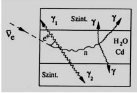
Figure 2: Schematic representation of the experimental set up used by Cowan and Reines to demonstrate the existence of the antineutrino.
