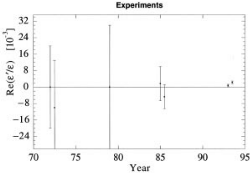
Figure 41: Results of the experiments that measure the possible contribution of direct CP violating contributions in the decay of kaons. It is seen that the experimental accuracy dramatically improves over time.
