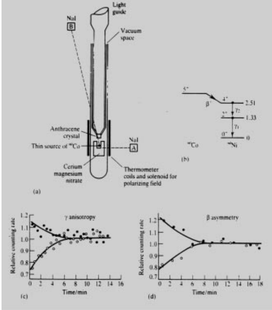
Figure 4: (a) Experimental set up used by Wu and collaborators to demonstrate the violation of parity in \beta -decay of ^{60}\text{Co} ; (b) Schematic representation of ^{60}\text{Co} Gamow-Teller decay; (c) Photon asymmetry measured with detector A ( \bullet ) and detector B ( \circ ) as function of time as the crystal warms; the difference between the curves is a measure of the net polarization of the nuclei; (d) \beta -asymmetry in the counting rates measured with the anthracene crystal for two directions of the magnetic field ( \bullet , down \downarrow ; \circ , up \uparrow ).
