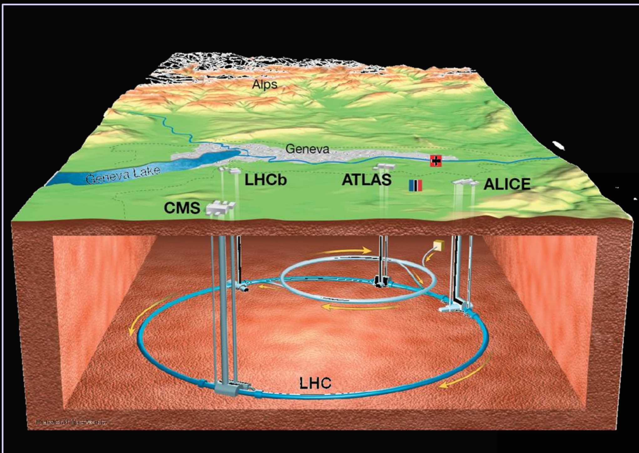
CERN LHC
