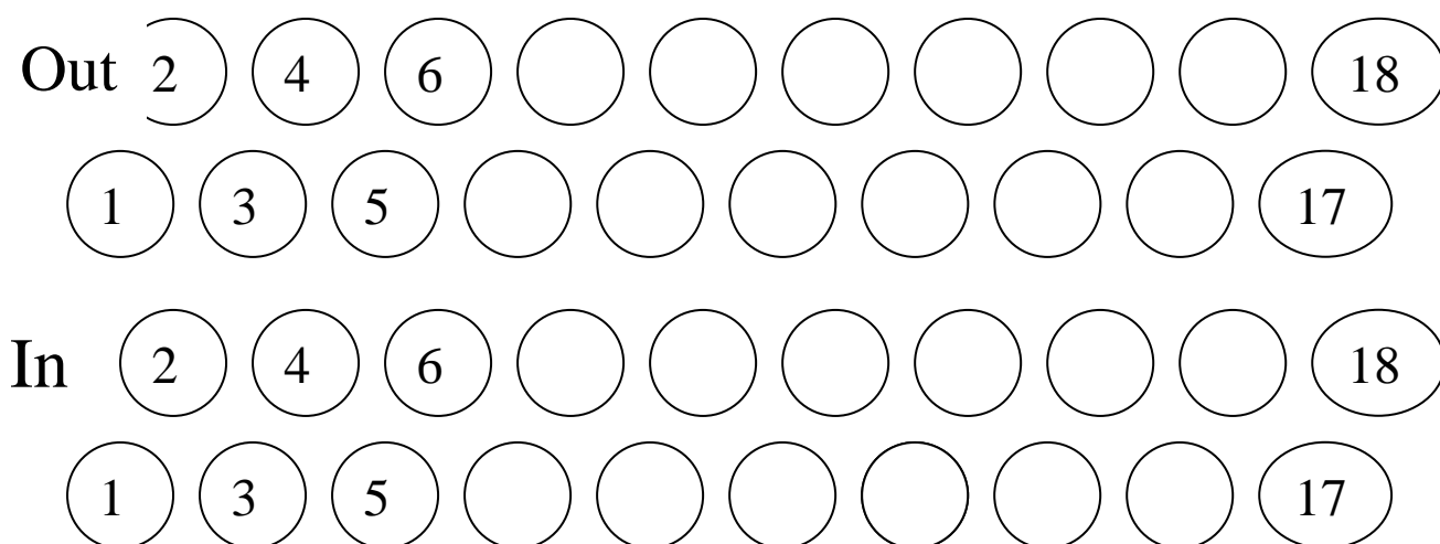
Figure 2: Top view of input and output channels at the distribution rack of side C.
