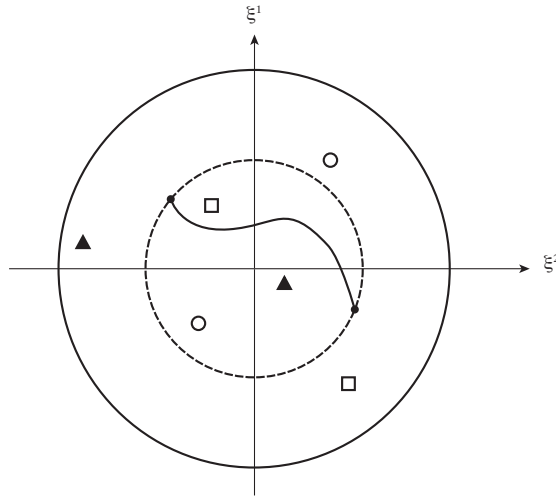
Figure C.1: Slice of the parameter space of the group SU(2) with \xi^3 = 0 . The origin corresponds to the identity \mathbf{I} . The boundary is a circle with radius 2\pi , which corresponds to the SU(2) element g = -\mathbf{I} . Each element inside the inner circle, which has radius \pi has a corresponding element in the outer region which differs by an overall minus sign according to (C.35). Three pairs of such points are indicated. The solid curve connecting two opposite points on the inner circle corresponds to a continuous set of SU(2) transformations with endpoints corresponding to two transformations differing by an overall sign. The parameter space of SO(3) can be imbedded in the same plot and covers only the inside of the circle with radius \pi . Two opposite points on the inner circle correspond to identical SO(3) elements. The SO(3) elements corresponding to the solid curve therefore describe a closed continuous set of SO(3) transformations.
