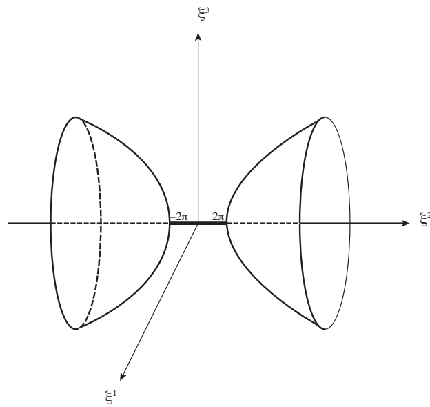
Figure C.2: The parameter space of the group \text{Sl}(2, \mathbb{R}) . The origin corresponds to the identity \mathbf{I} . The boundary is a hyperboloid which corresponds to the \text{Sl}(2, \mathbb{R}) element g = -\mathbf{I} . Elements corresponding to the line with \xi^2 between -2\pi and 2\pi and \xi^1, \xi^3 = 0 constitute the (compact) subgroup \text{SO}(2) .
