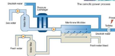
PRO – pressure retarded osmosis
