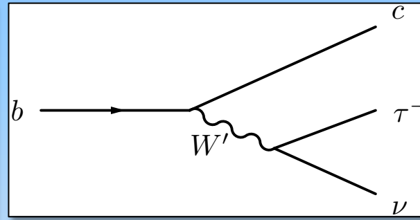
SU(2)'
