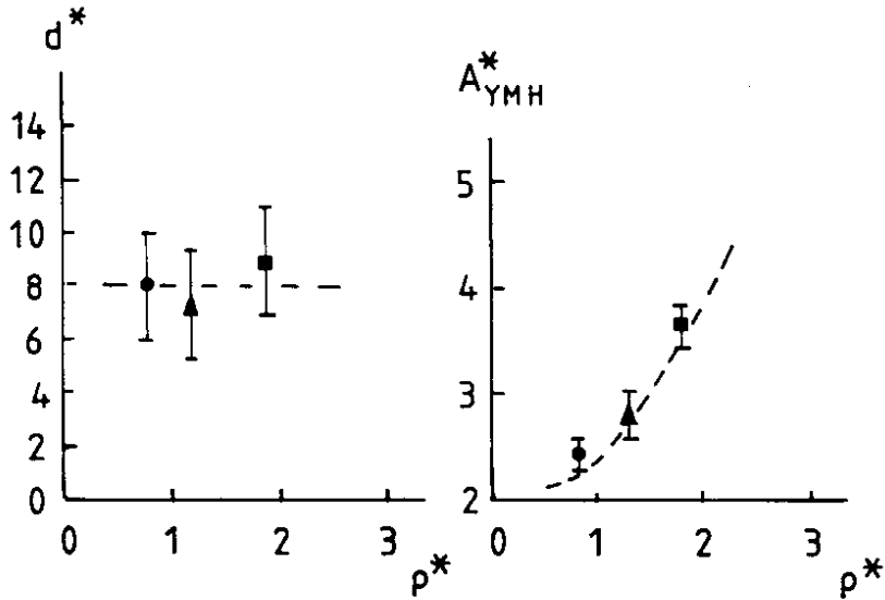
Figure 2: Estimates of the distance parameter d^* and corresponding action A_{\text{YMH}}^* of the new instanton I^* , both as a function of its scale \rho^* . The distances d^* and \rho^* are in units M_W^{-1} and the action A_{\text{YMH}}^* in units 2\pi/\alpha_w . The dashed curves are the parametrization (7).
