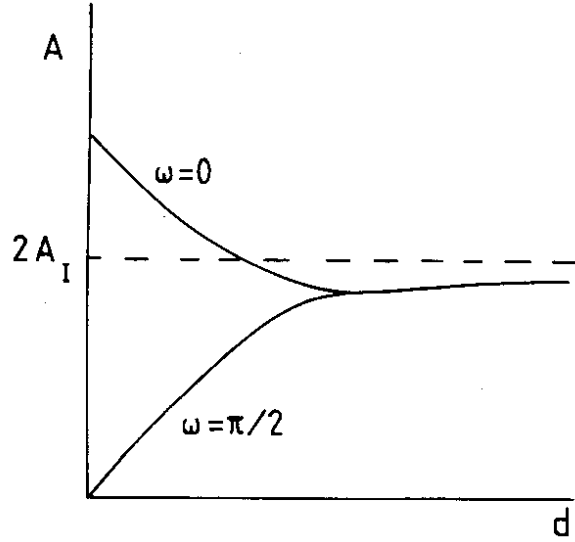
Figure 1: Sketch of the action A vs. the core separation d for the configurations in the repulsive ( \omega = 0 ) and attractive ( \omega = \pi/2 ) Yang-Mills channels, at vanishing Higgs coupling constant \lambda = 0 . The action is understood to include a higher dimension term (6), with given Lagrange multiplier, to fix the scale.
