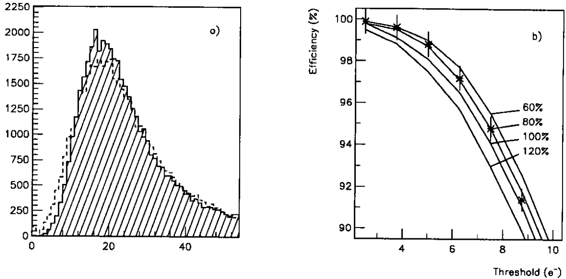
Figure 4: a) Calculated signal from an MSGC assuming very low gain fluctuations (hatched histogram) and high gain fluctuations (dashed line). b) The calculated efficiency of an MSGC as a function of the applied threshold for different values of the gain fluctuation RMS; as a comparison, a few measured points are plotted from the beam test.
