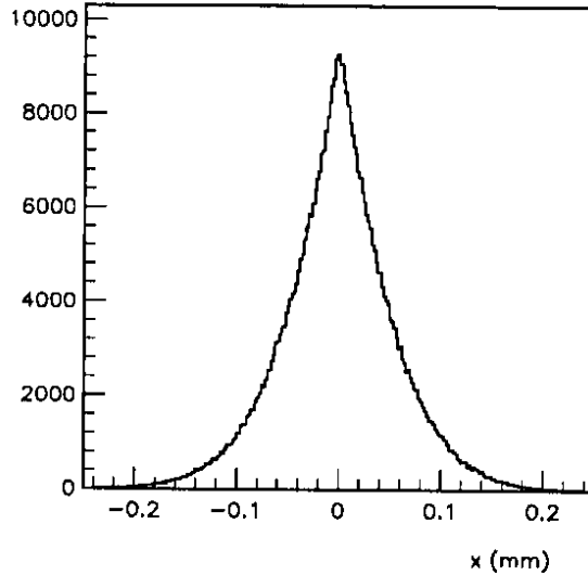
Figure 2: Distribution of electrons along the x -direction after drift and diffusion, for a 5 mm gas gap and \sigma_T = 50 \mu\text{m}/\sqrt{\text{mm}} .
