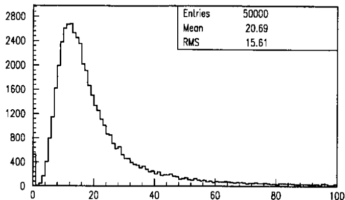
Figure 3: Total ionisation spectrum in a typical MSGC using DME/CO 2 60/40 with an estimated cluster size distribution (see text).
