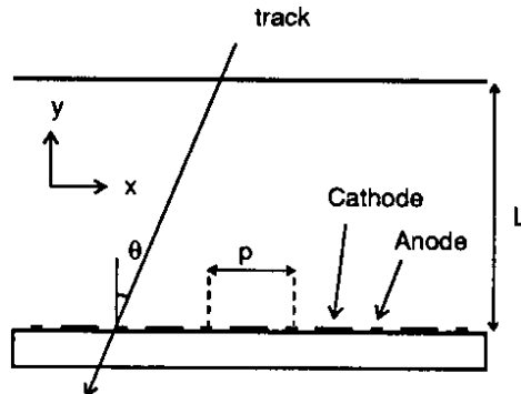
Figure 1: Geometry of the MSGC.
