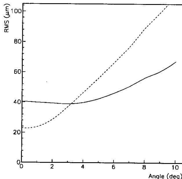
Figure 6: The position resolution of an MSGC as a function of the angle of incidence of the ionising track, for an MSGC with 2 mm gas gap (solid line) and in case of a 5 mm gas gap (dashed line), both with a 200 \mu\text{m} pitch.
