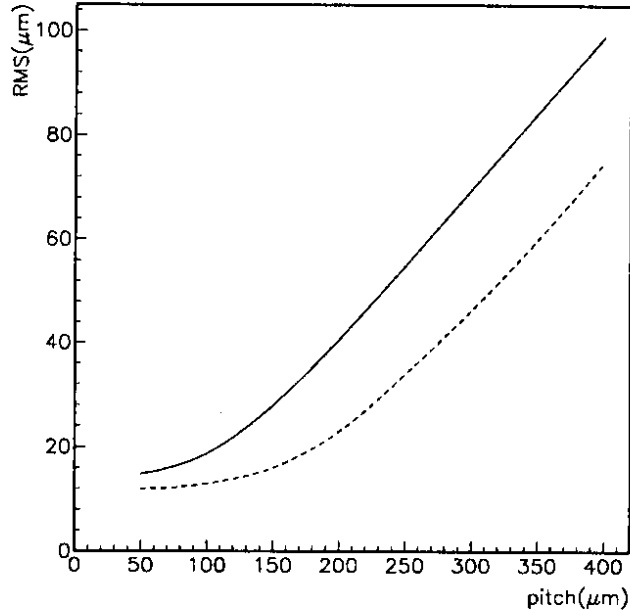
Figure 7: The position resolution of an MSGC as a function of the anode pitch for an MSGC with L = 2 \text{ mm} (solid line) and L = 5 \text{ mm} (dashed line).
