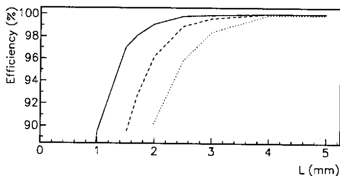
Figure 8: The efficiency of a 200 \mu\text{m} pitch MSGC as a function of the gas gap width L , with a threshold on the highest strip of 1.9 electrons (solid line), 3.8 (dashed line) and 5.7 (dotted line).
