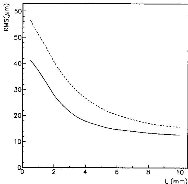
Figure 5: The position resolution of an MSGC as a function of the gap thickness L with p = 150 \mu\text{m} (solid line) and p = 200 \mu\text{m} (dashed line).
