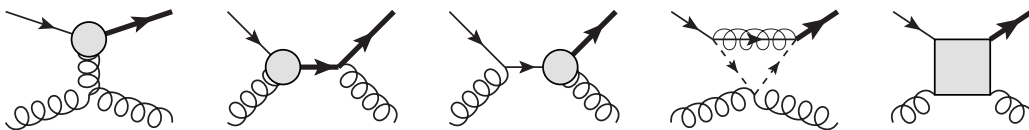
Figure 2: Feynman diagrams contributing to ug \rightarrow tg . The shaded t - u - g vertex represents the diagrams in Figure 1. Cross-channel gluon diagrams are not shown.
