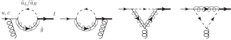
Figure 1: The bubble and triangle diagrams contributing to the t - u - g FCNC. The arrows on the gluino lines are indicative of their Dirac fermion nature.
