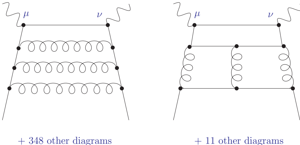
Figure 1: Typical Feynman diagrams for the contributions without (left) and with (right) d^{abc}d_{abc} to the charged-current DIS coefficient function C_3^- up to the third order in the strong coupling \alpha_s .
