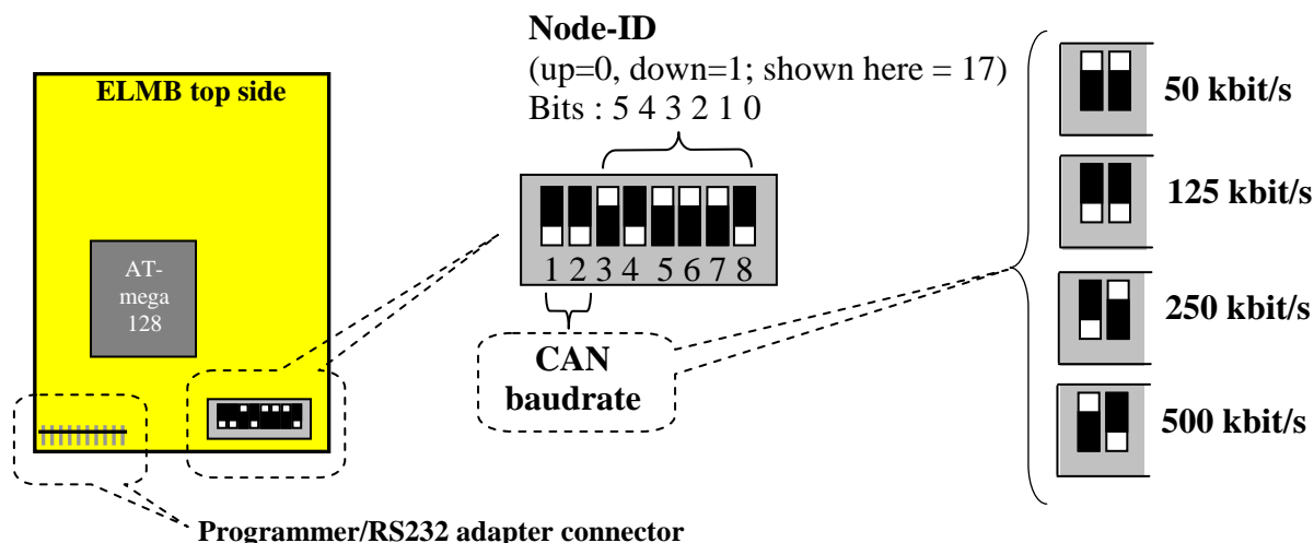
Figure 1. Location and function of ELMB DIP-switches (to set NodeID and CAN bus baudrate) and the location of the 10-pin Programmer/RS232 adapter connector..
