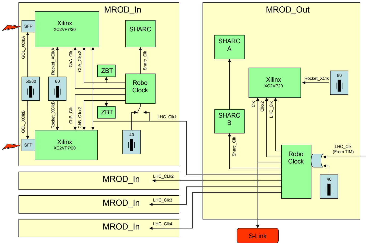
MROD-X Clocks
