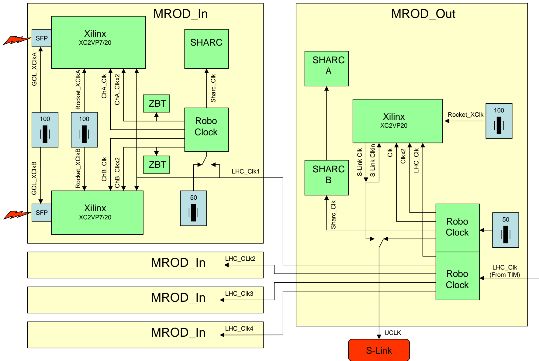
MROD-X Clocks
